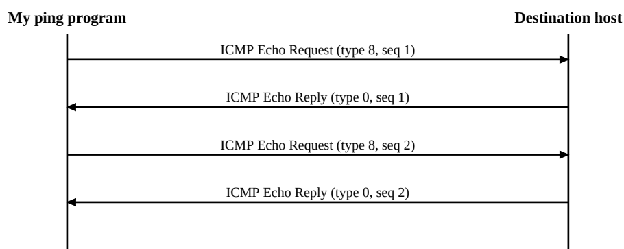
Fig 2: Working of the ping program
